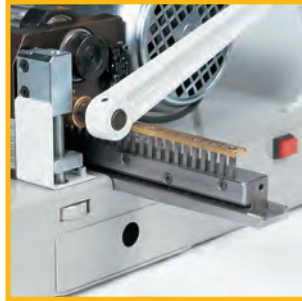
Punching tool.
